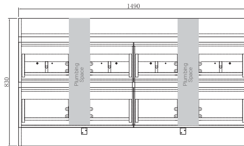
MIA 150D Front Section
