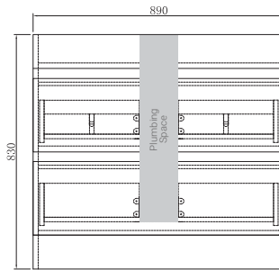
MIA 90 Front Section
