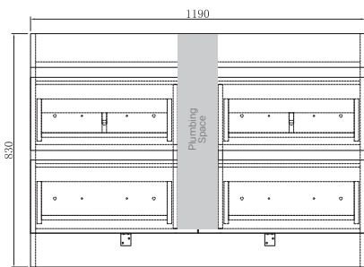
MIA 120S Front Section
