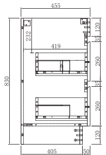
ALL SIZES Side Section
