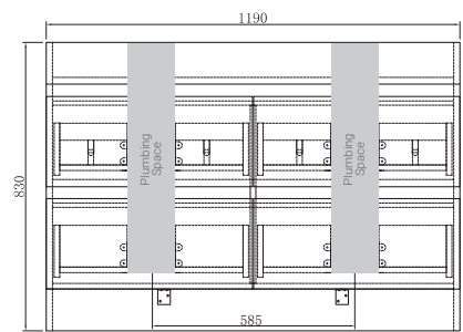
MIA 120D Front Section
