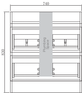
MIA 75 Front Section
